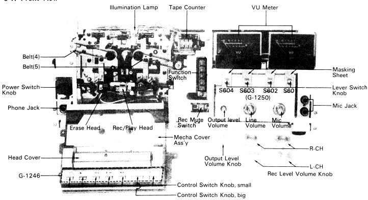
6-1. Front View
