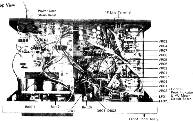
6-2. Top View
